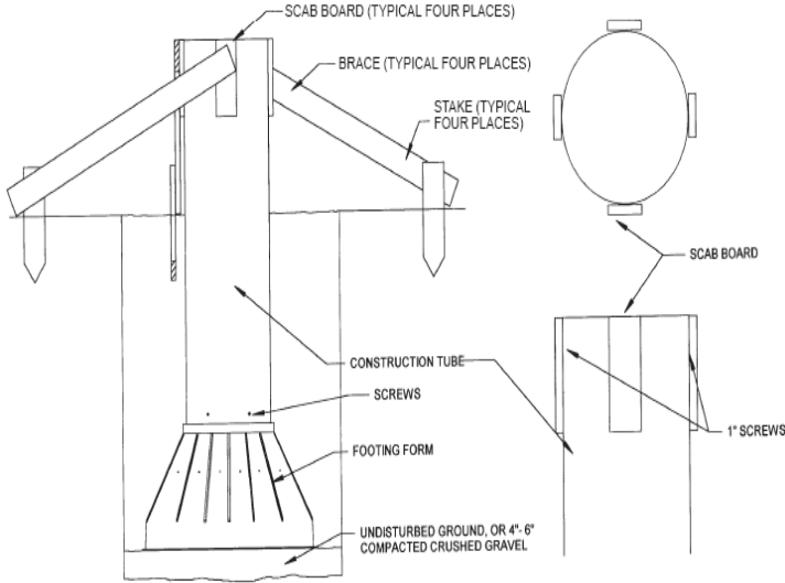
FIGURE 2—TYPICAL BRACING DURING CONSTRUCTION
