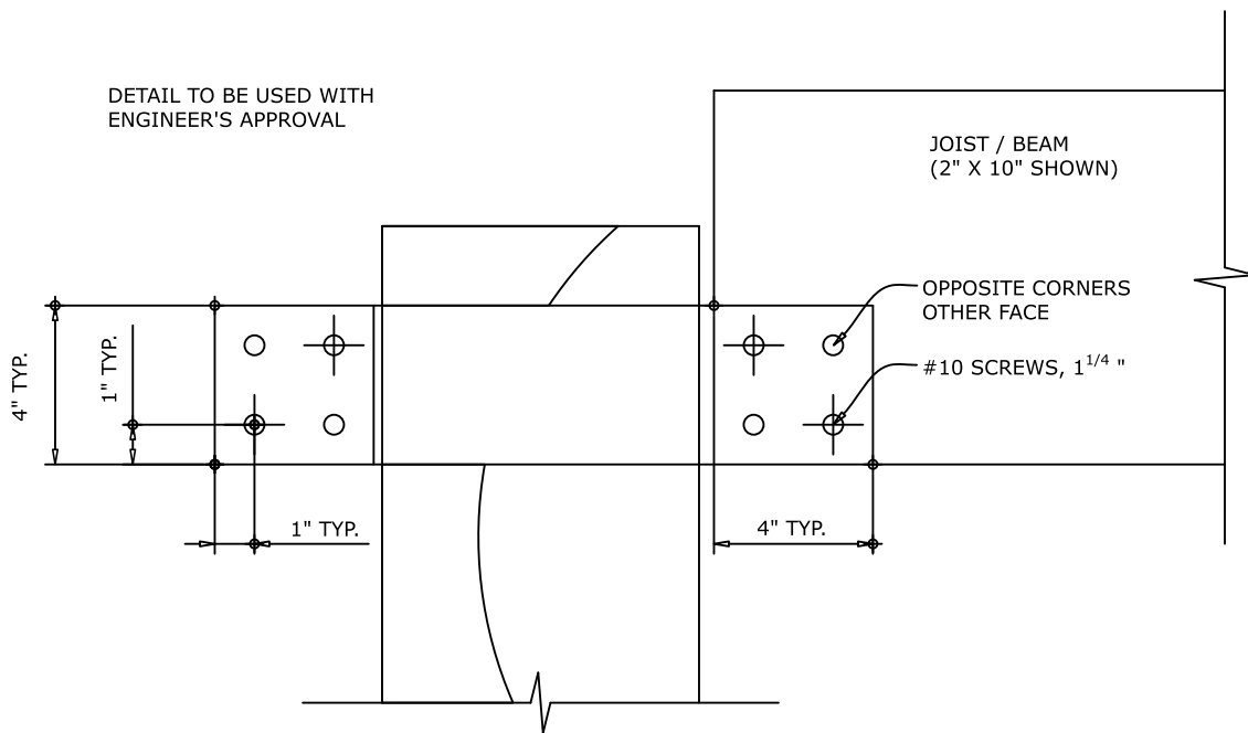
FRONT VIEW
